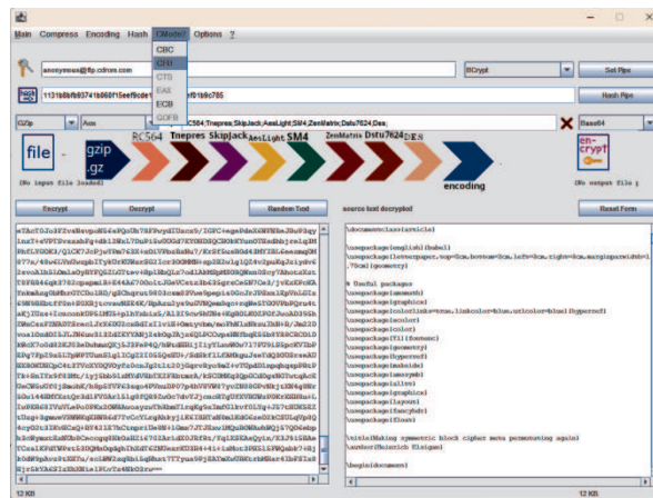
Figure 5: javafx.swing.JFrame.java
